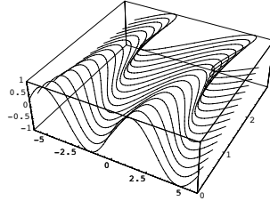
The family of \pi_2^{-1}(t) \cap W(\mathcal{L})
