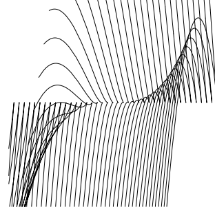
Fig.7: (6) Mixed fold
