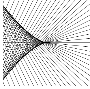
Fig.6: (5) Clairaut cusp
