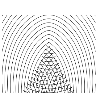
Fig.5: (4) Regular cusp
