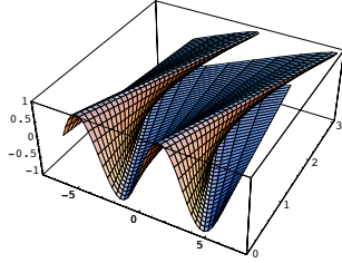
The graph of the geometric solution of Burger's equation
