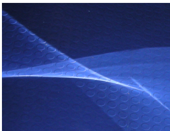
Fig.4: The caustic reflected by a mirror
